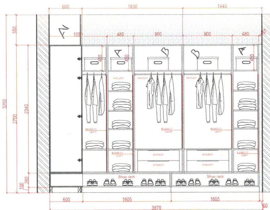
Front Elevation-A Details
