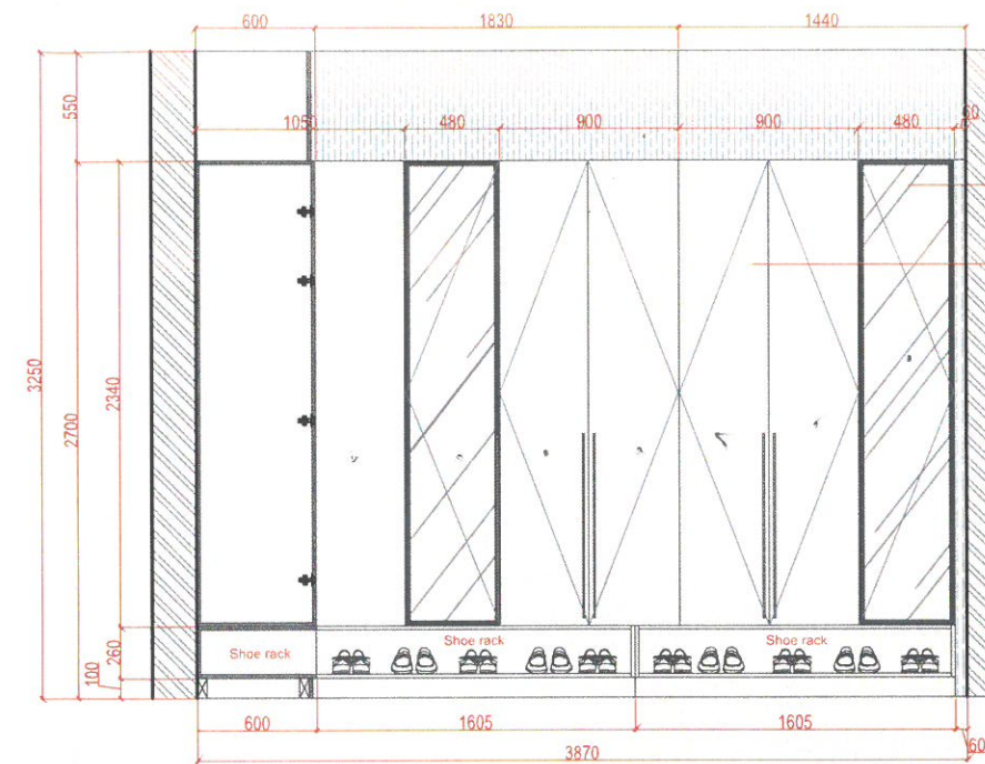
Front Elevation-A Details with Doors
