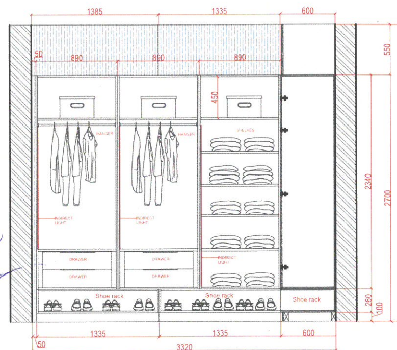
Front Elevation-B Details
