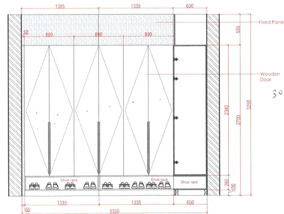
Front Elevation-B Details with Doors
